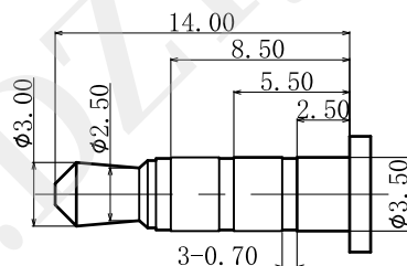
(3.50mm 4 POLE PLUG DETAIL DRAWING)
