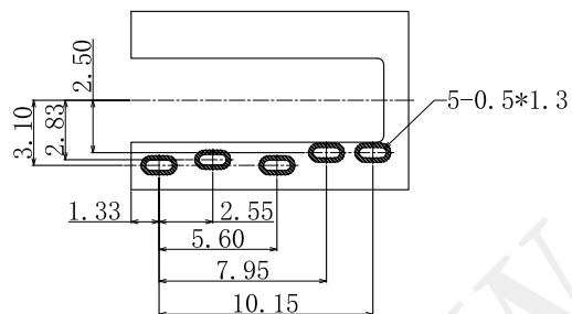
P.C.B LAYOUT (All SIZES \pm 0.05 mm) TOP VIEW
