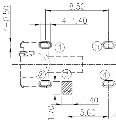
RECOMMENDED PCB LAYOUT (TOP VIEW) GENERAL TOLERANCES: ±0.05
