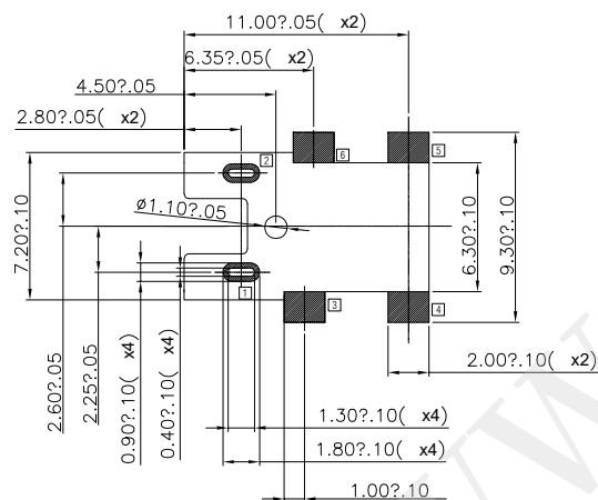
RECOMMEND PAD LAYOUT
