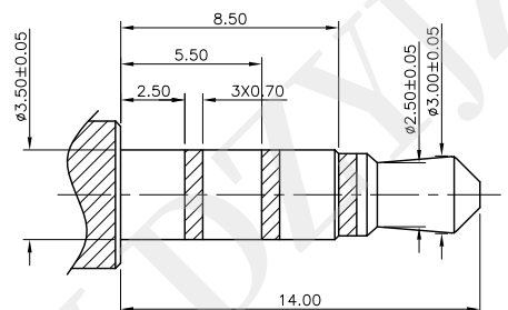
(0.350mm 3 OR 4 POLE PLUG DETAIL DRAWING)
