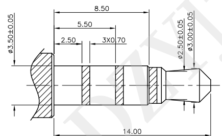
(0.350mm 3 OR 4 POLE PLUG DETAIL DRAWING)
