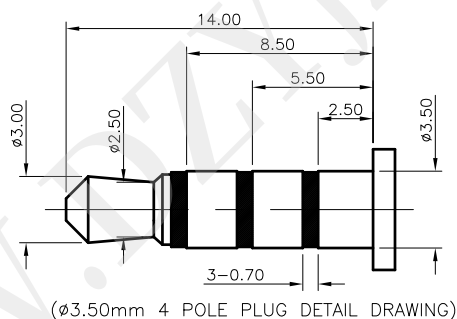
(3.50mm 4 POLE PLUG DETAIL DRAWING)
