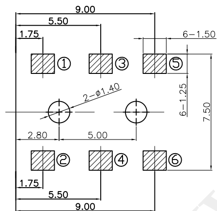
RIGHT PACKING P.C.B LAYOUT TOP VIEW
