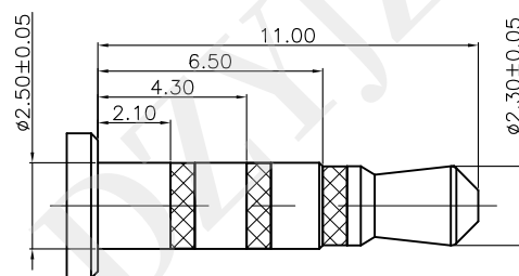
2.50mm 4 POLE PLUG DETAIL DRAWING)
