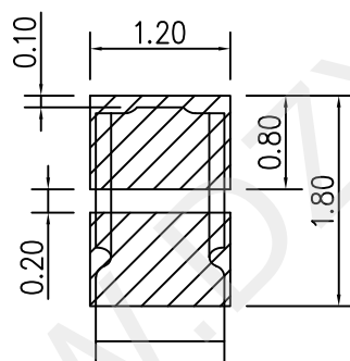
METAL MASK T=0.10 TOLERANCE±0.05 (钢网推荐图) (FOR REFERENCE ONLY)
