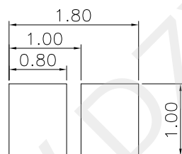
METAL MASK T=0.08 TOLERANCE±0.05(钢网推荐图) (FOR REFERENCE ONLY)
