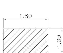
RECOMMENDED PCB LAYOUT TOLERANCE±0.05(焊盘推荐图) (FOR REFERENCE ONLY)
