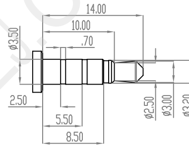
φ 3.50mm 4 POLE PLUG DETAIL DRAWING(2/1)
