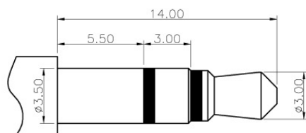
Ø3.50mm 3 POLE PLUG
