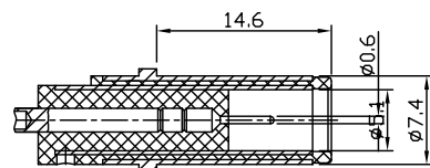
RECOMMENDED PLUG
