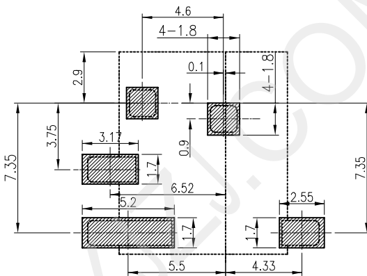
PCB LAYOUT TOP VIEW TOLERANCES: 2.05
