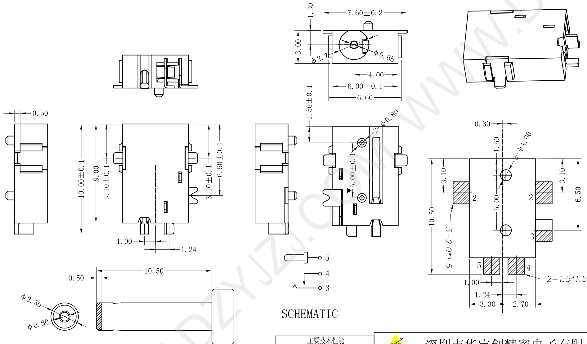
∅2.5mm 2 POLE PLUG DETAIL DRAWING
