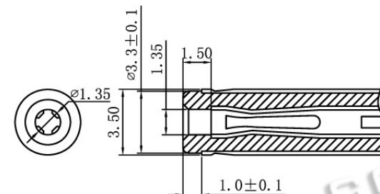
MATE PLUG
